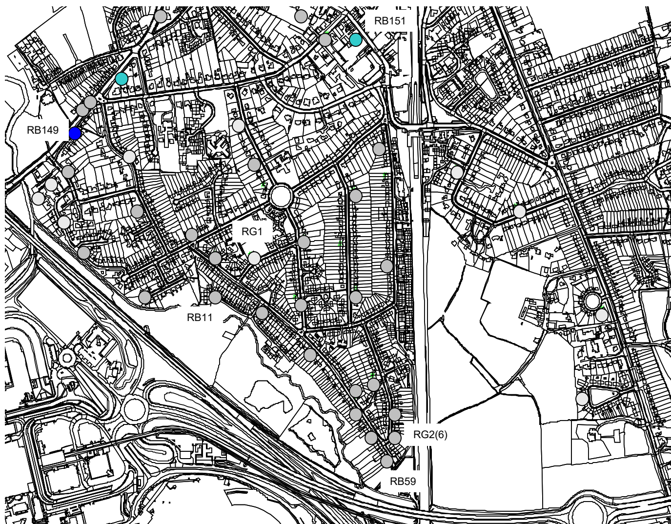
Figure 1: Monitoring Results for Nitrogen Dioxide Concentrations across the Horley Gardens Estate in 2025. Tube Correction Factor = 0.87 (n=11 min).
