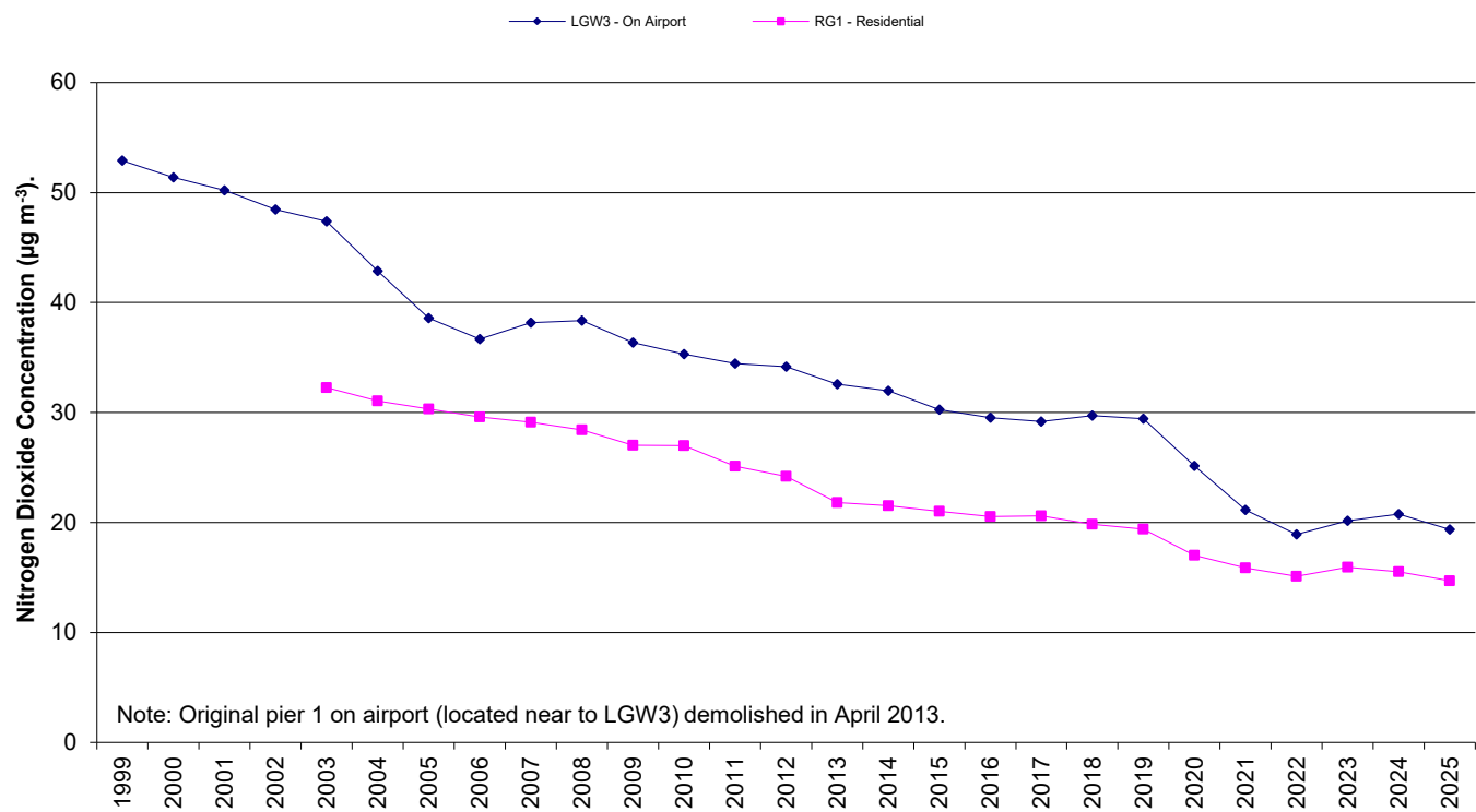
Figure 4: Three Year Rolling Annual Average Nitrogen Dioxide Concentration at LGW3, Gatwick Airport.
